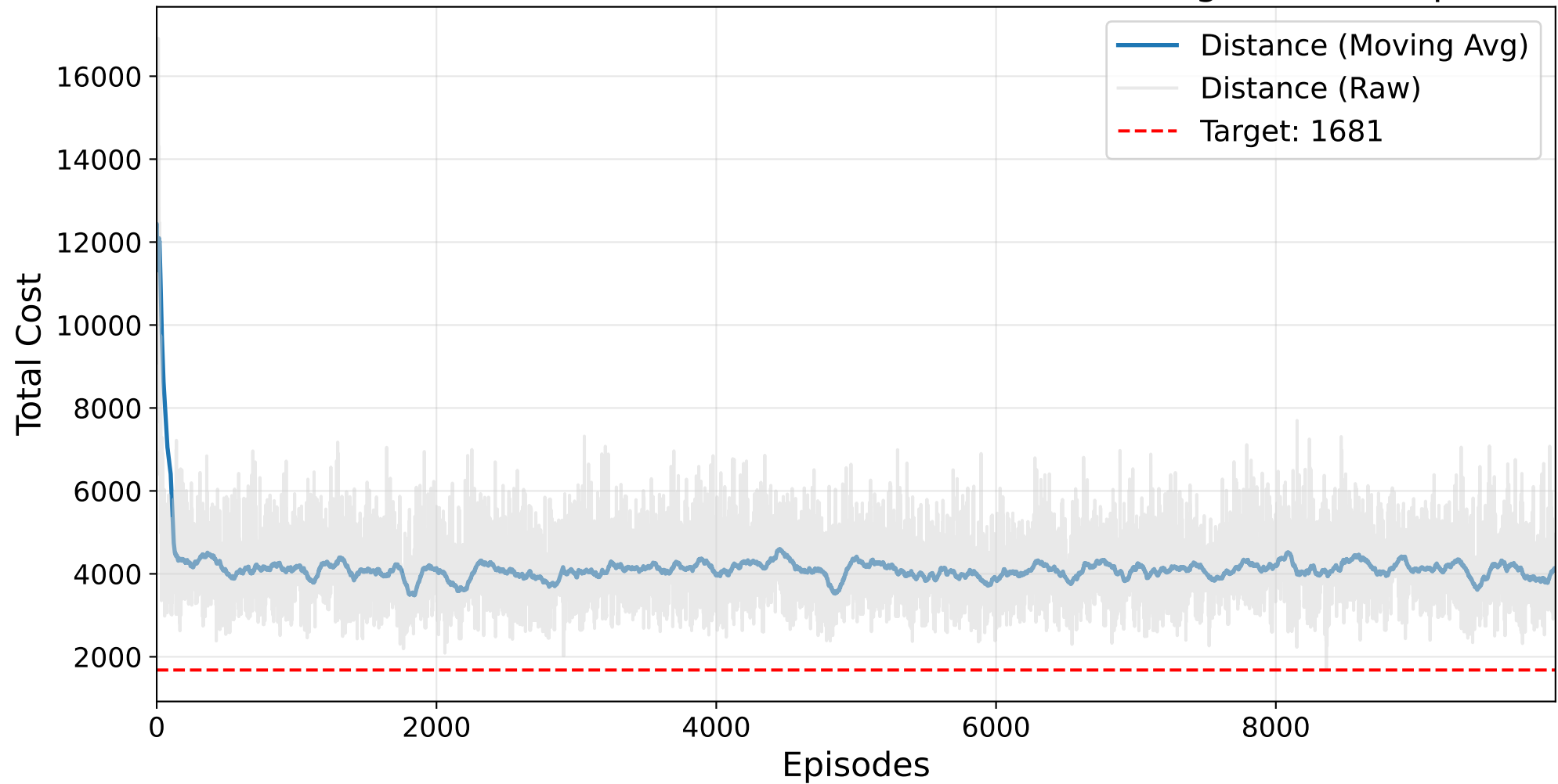
Final HYPERBAND TPE Masked AutoRL-SOP Training - ESC25.sop
